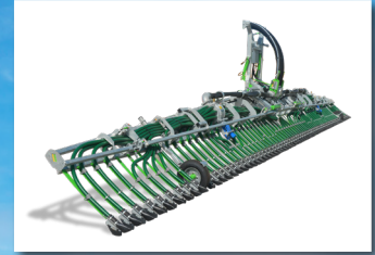
PENDSLIDE PRO 150/60PS2 15-m spreading boom
