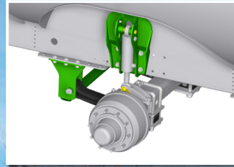
Hydro-Tandem: hydraulic axle suspension
